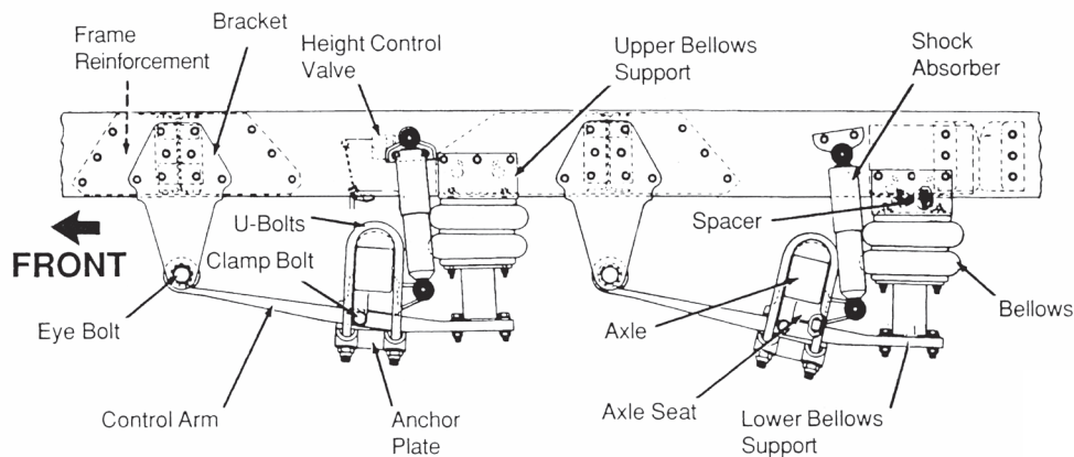
Figure 2.4 Air Suspension Parts
