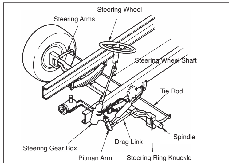
Figure 2.1 Steering System
